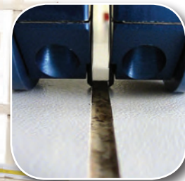
Scoring System
