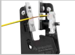
Positive stripping thanks to precise shape of the blades.
