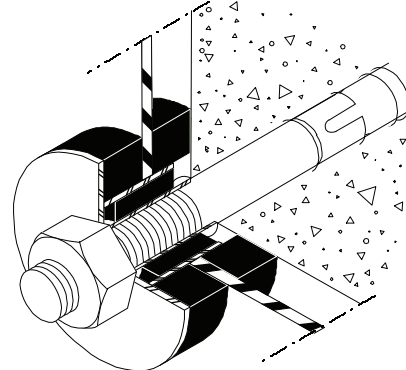
PB Mount with SAS Seismic Anchor Stud
