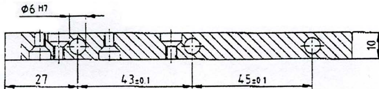
Base plate of Thermocutter ZETZ-25 with mounting holes (dimensions in mm)
